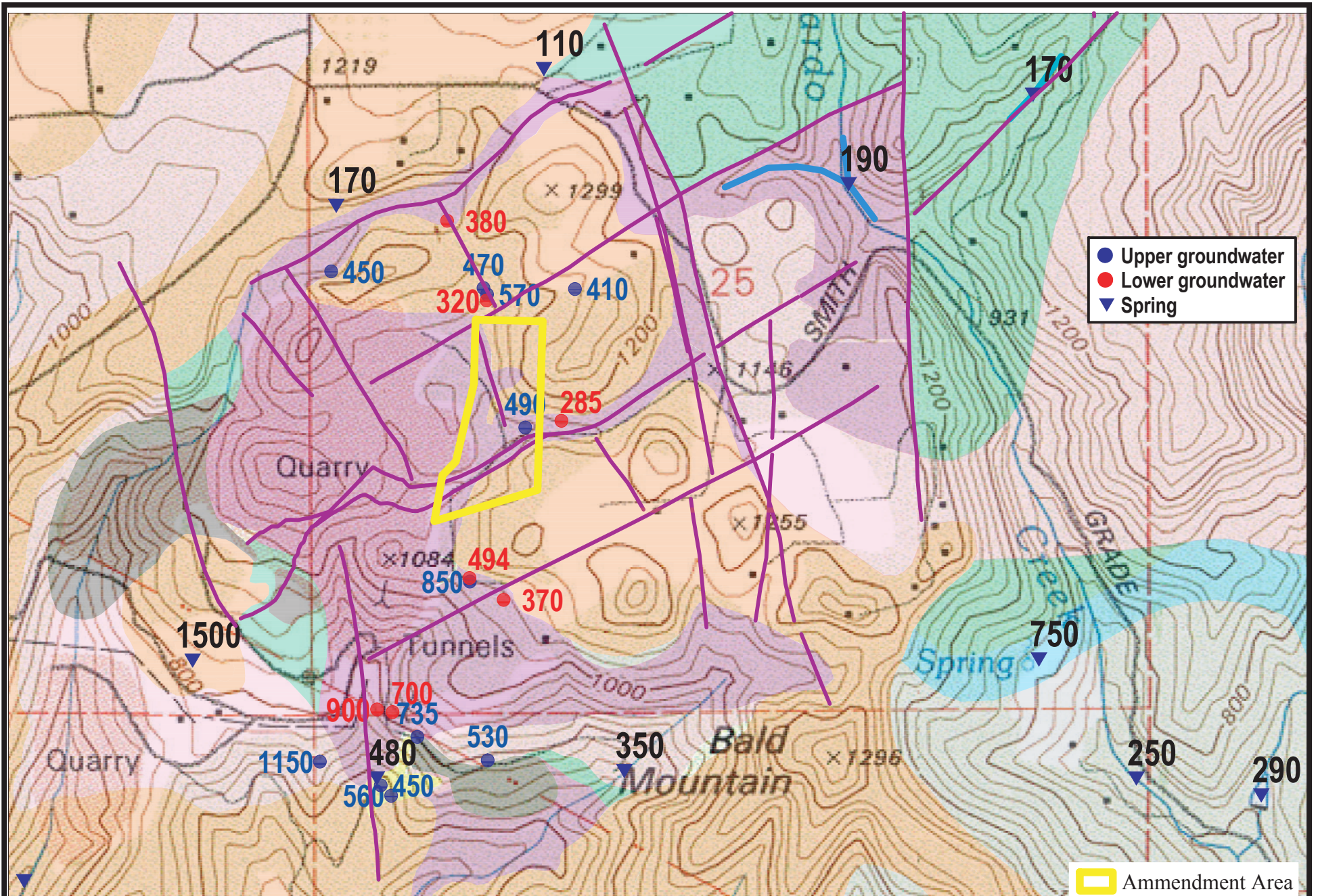
Average Specific Conductance, Groundwater and Springs (uS/cm)
